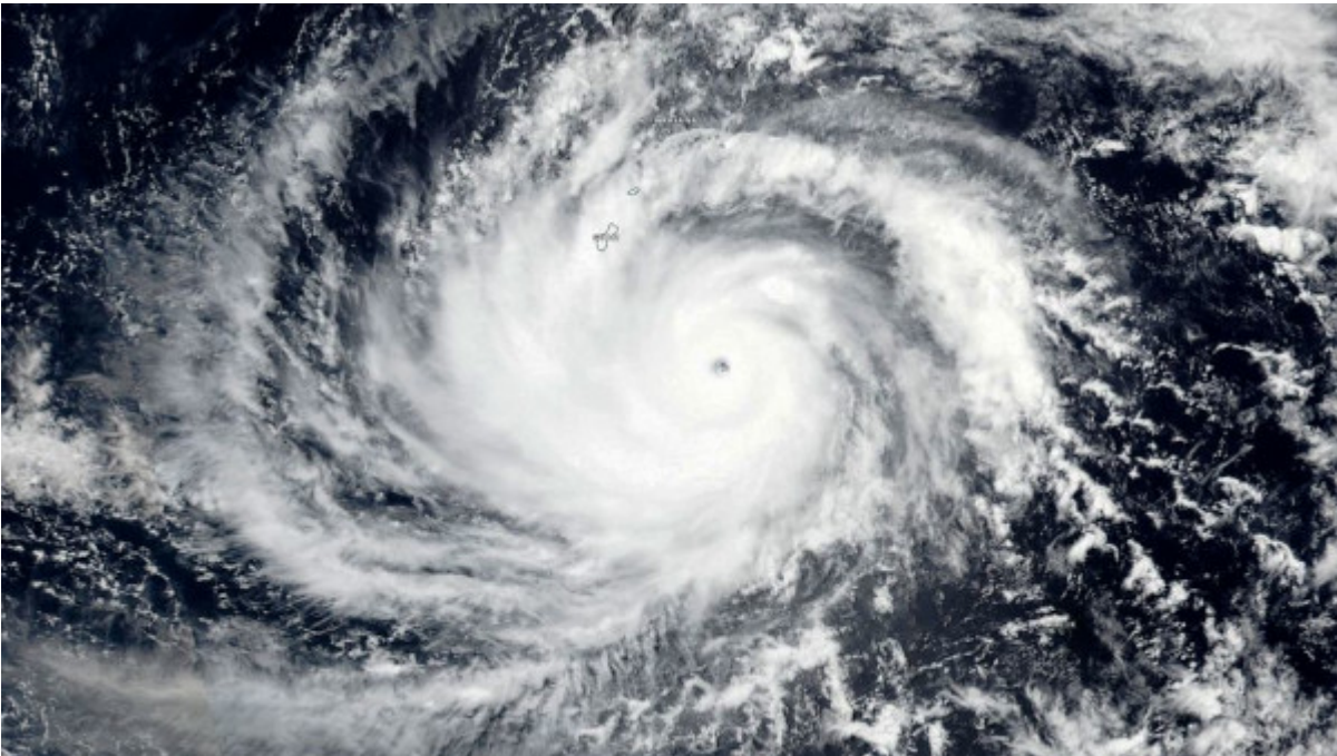
Typhoon Mawar in the Northern Western Pacific near Guam.
